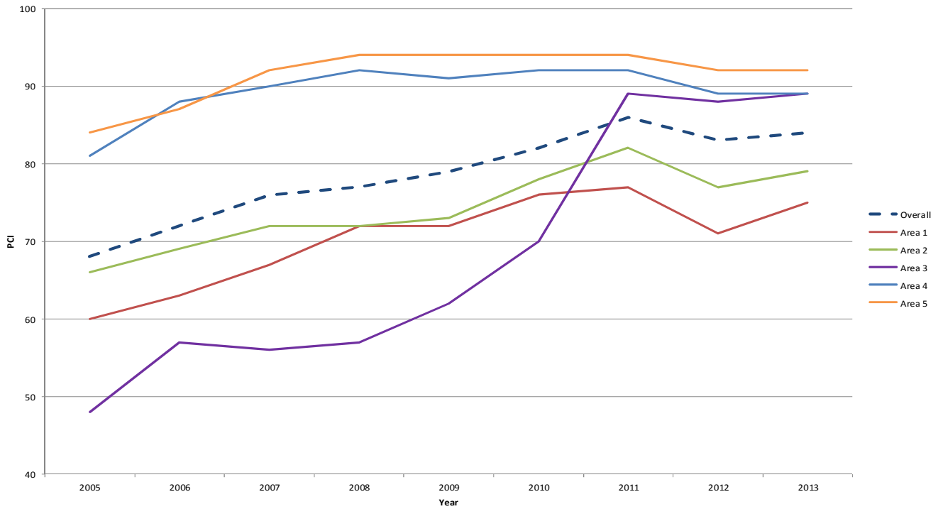
Pavement Condition Index (PCI) vs Year
